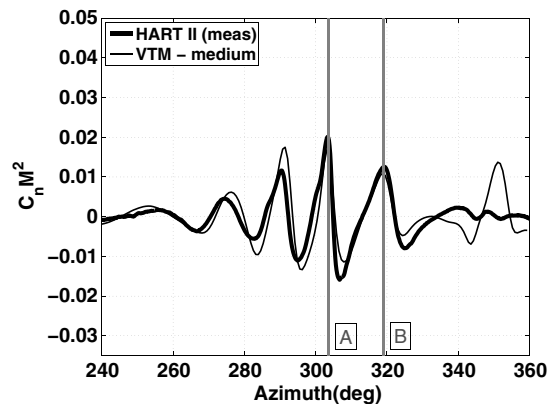
Fig. 6 Time history of acoustic pressure for one blade passage and the corresponding BVI-induced airloads and source density distribution on the rotor for an observer (marked by small circle) located at the experimentally measured SPL maximum on the retreating side of the rotor (HART II BL case). Numerical results are for the medium computational resolution.
