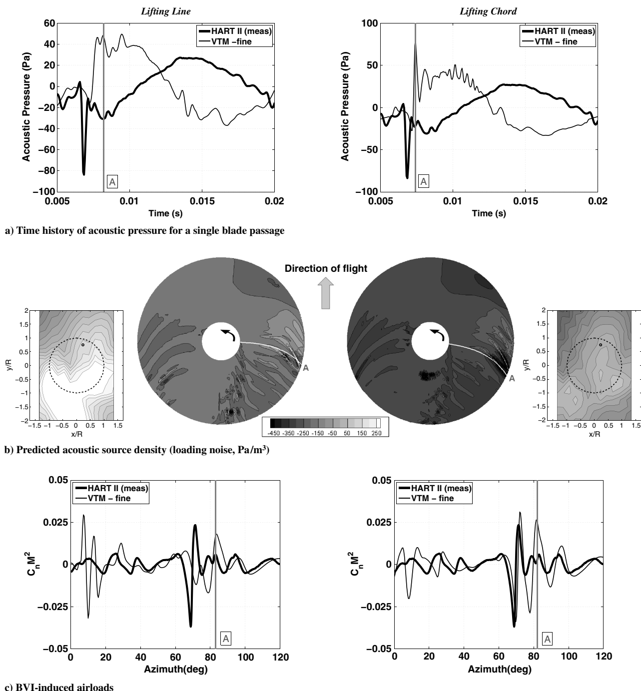
Fig. 17 Time history of acoustic pressure for one blade passage and the corresponding BVI-induced airloads and source density distribution on the rotor for an observer (marked by small circle) located at the experimentally measured SPL maximum on the advancing side of the rotor (HART II MN case). Numerical results are for the fine computational resolution.
