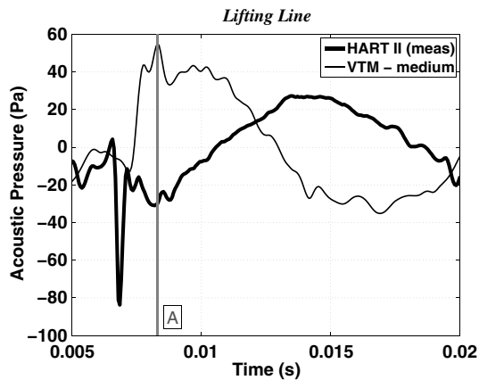
a) Time history of acoustic pressure for a single blade passage
