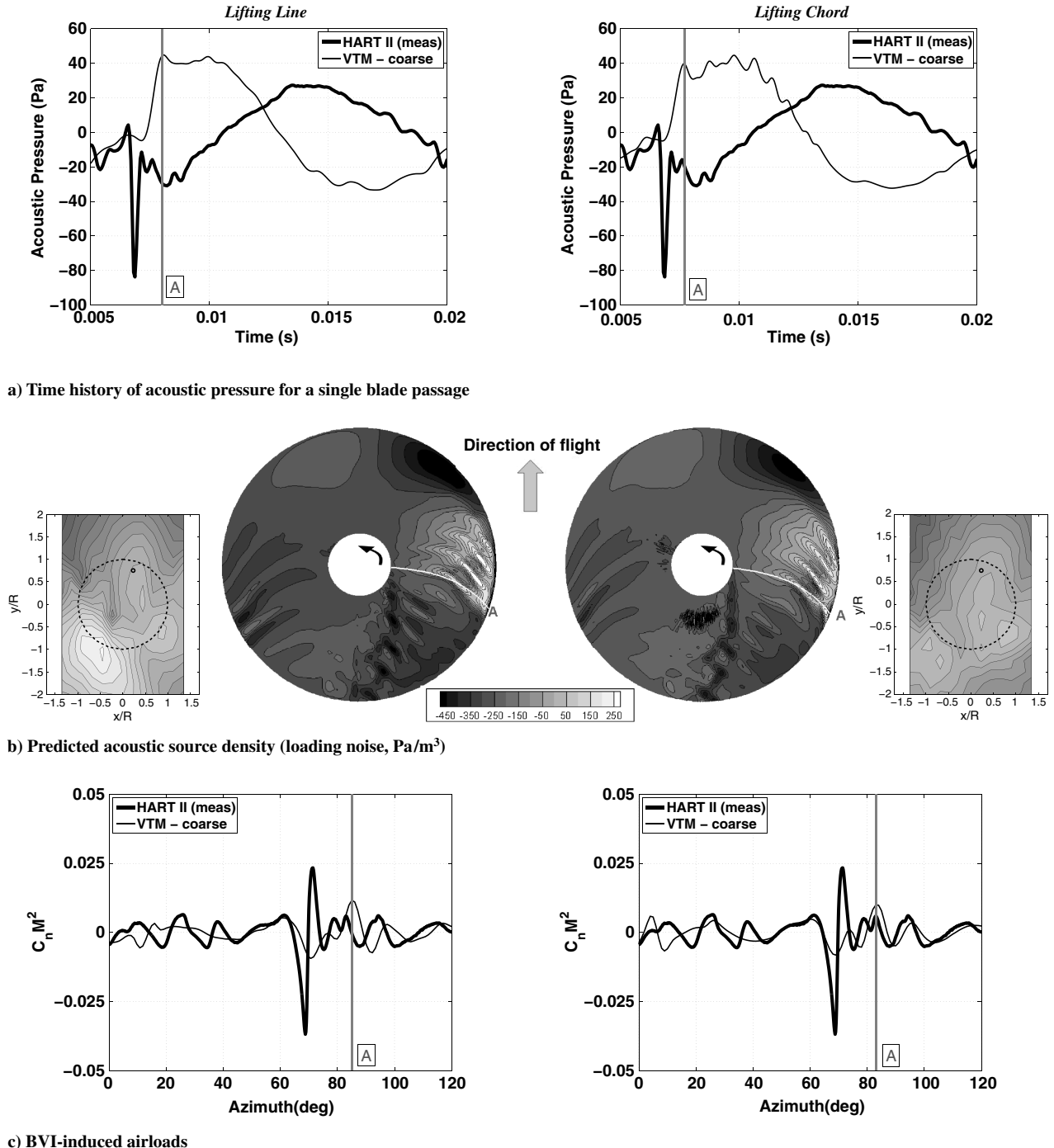
Fig. 15 Time history of acoustic pressure for one blade passage and the corresponding BVI-induced airloads and source density distribution on the rotor for an observer (marked by small circle) located at the experimentally measured SPL maximum on the advancing side of the rotor (HART II MN case). Numerical results are for the coarse computational resolution.
