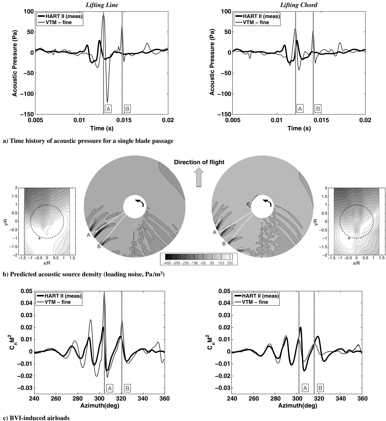
Fig. 7 Time history of acoustic pressure for one blade passage and the corresponding BVI-induced airloads and source density distribution on the rotor for an observer (marked by small circle) located at the experimentally measured SPL maximum on the retreating side of the rotor (HART II BL case). Numerical results are for the fine computational resolution.
