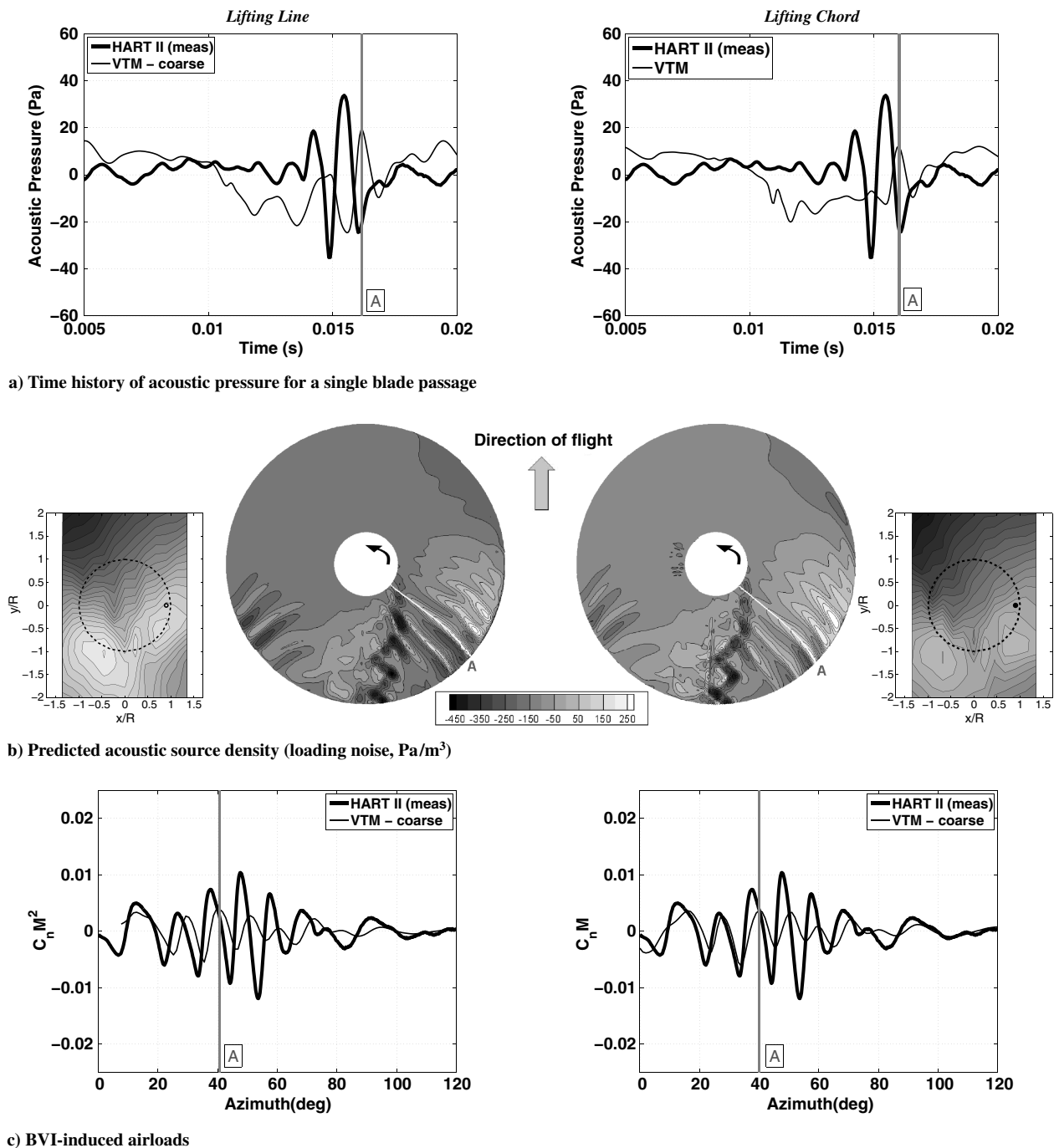
Fig. 8 Time history of acoustic pressure for one blade passage and the corresponding BVI-induced airloads and source density distribution on the rotor for an observer (marked by small circle) located at the experimentally measured SPL maximum on the advancing side of the rotor (HART II BL case). Numerical results are for the coarse computational resolution.
