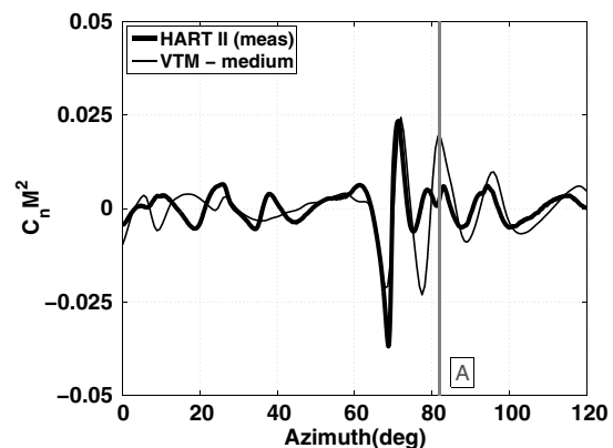
Fig. 16 Time history of acoustic pressure for one blade passage and the corresponding BVI-induced airloads and source density distribution on the rotor for an observer (marked by small circle) located at the experimentally measured SPL maximum on the advancing side of the rotor (HART II MN case). Numerical results are for the medium computational resolution.
