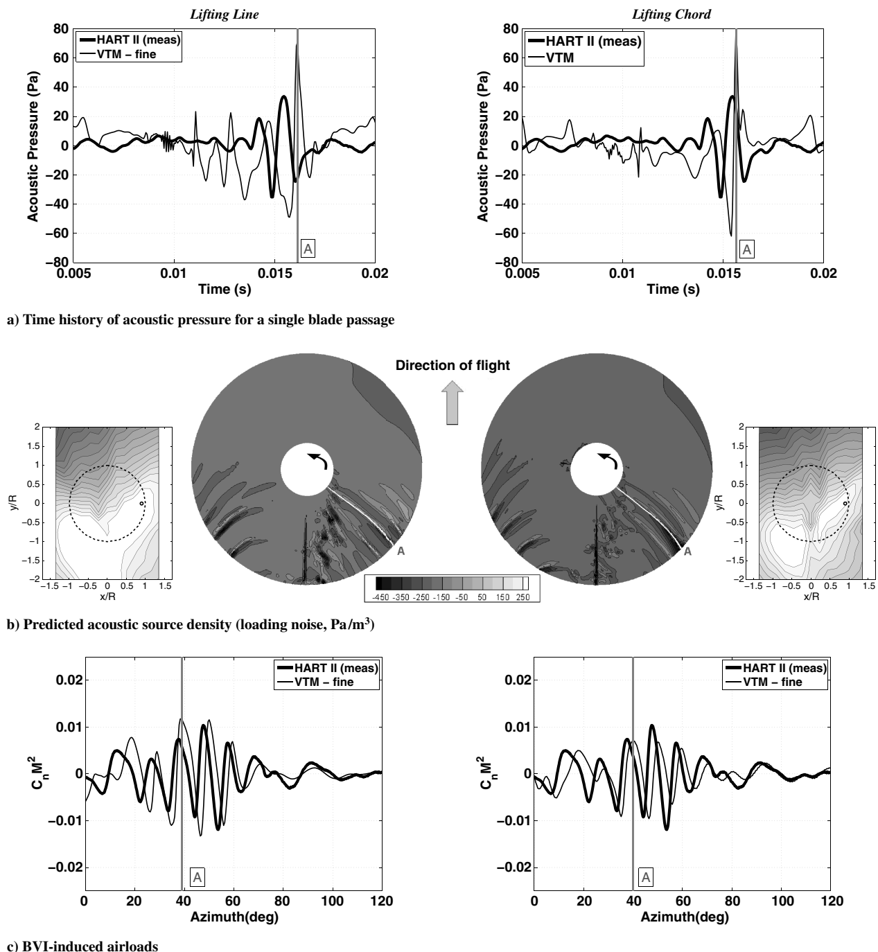
Fig. 10 Time history of acoustic pressure for one blade passage and the corresponding BVI-induced airloads and source density distribution on the rotor for an observer (marked by small circle) located at the experimentally measured SPL maximum on the advancing side of the rotor (HART II BL case). Numerical results are for the fine computational resolution.
