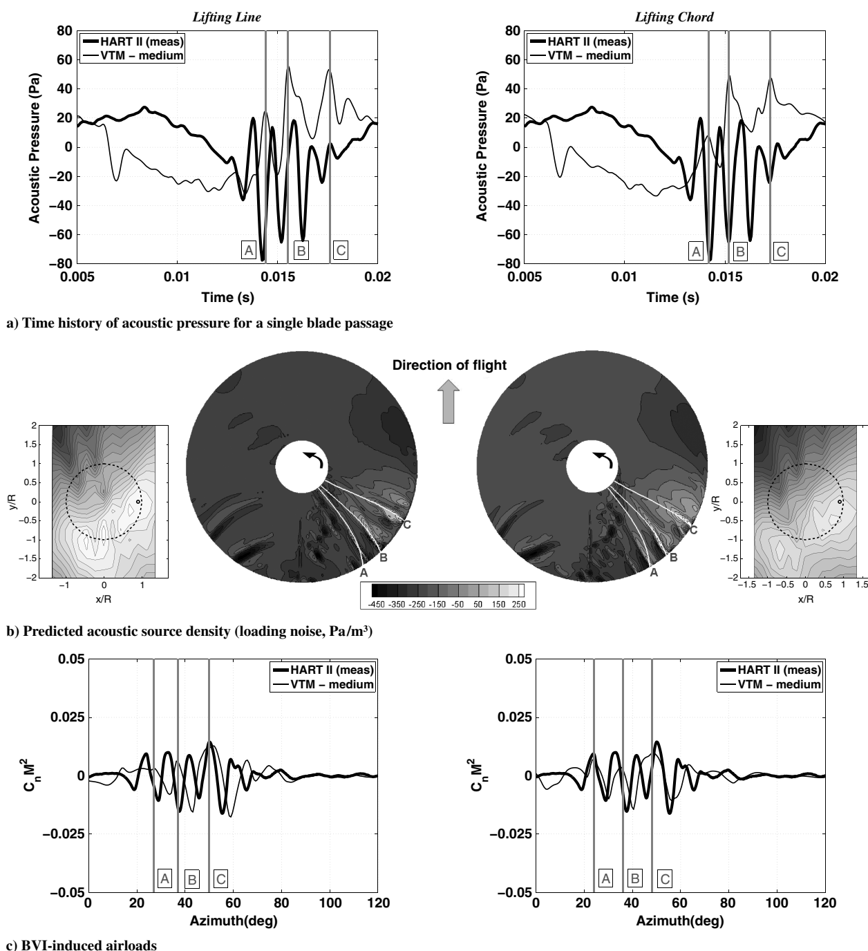
Fig. 23 Time history of acoustic pressure for one blade passage and the corresponding BVI-induced airloads and source density distribution on the rotor for an observer (marked by small circle) located at the experimentally measured SPL maximum on the advancing side of the rotor (HART II MV case). Numerical results are for the medium computational resolution.
