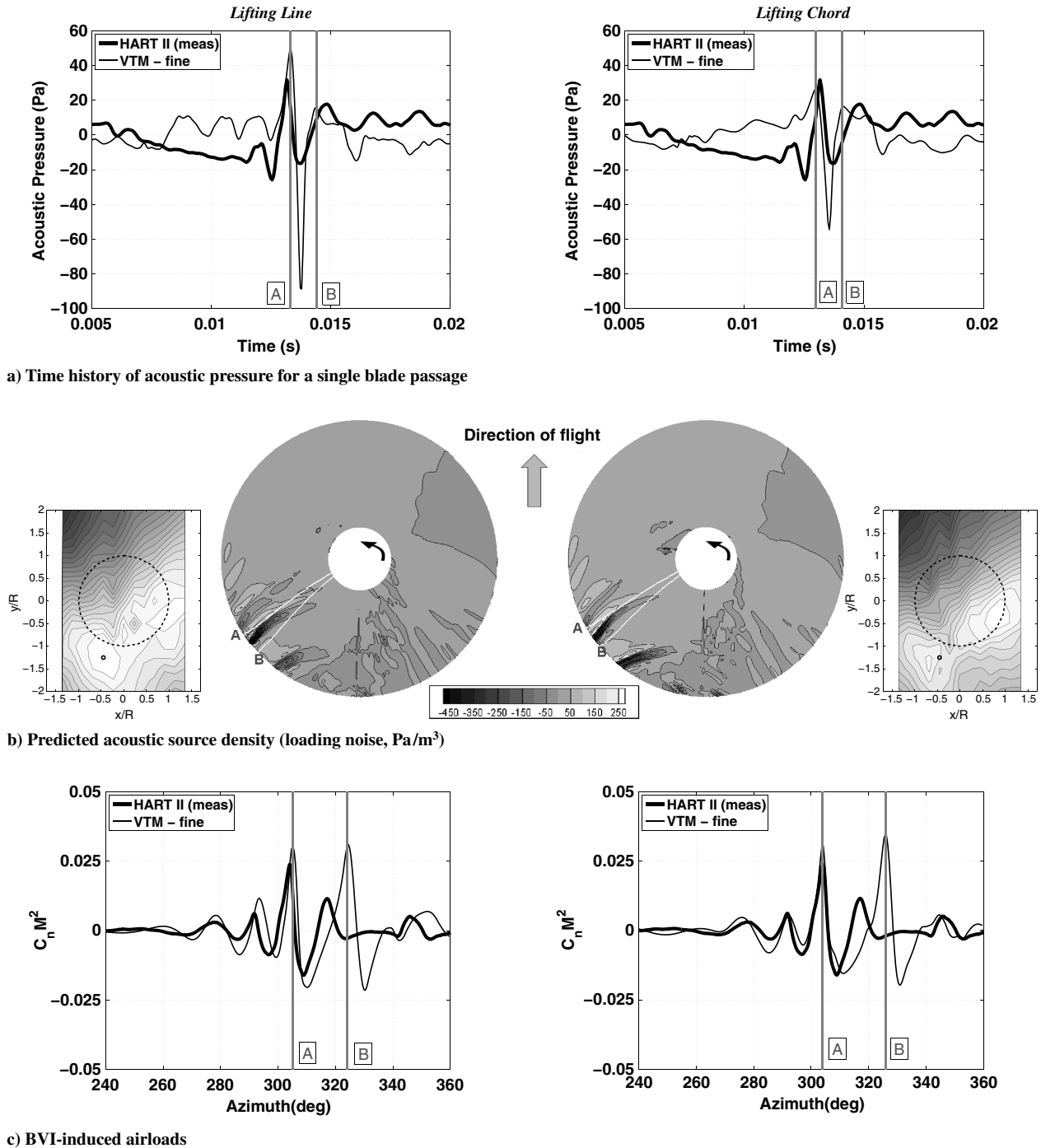
Fig. 21 Time history of acoustic pressure for one blade passage and the corresponding BVI-induced airloads and source density distribution on the rotor for an observer (marked by small circle) located at the experimentally measured SPL maximum on the retreating side of the rotor (HART II MV case). Numerical results are for the fine computational resolution.
