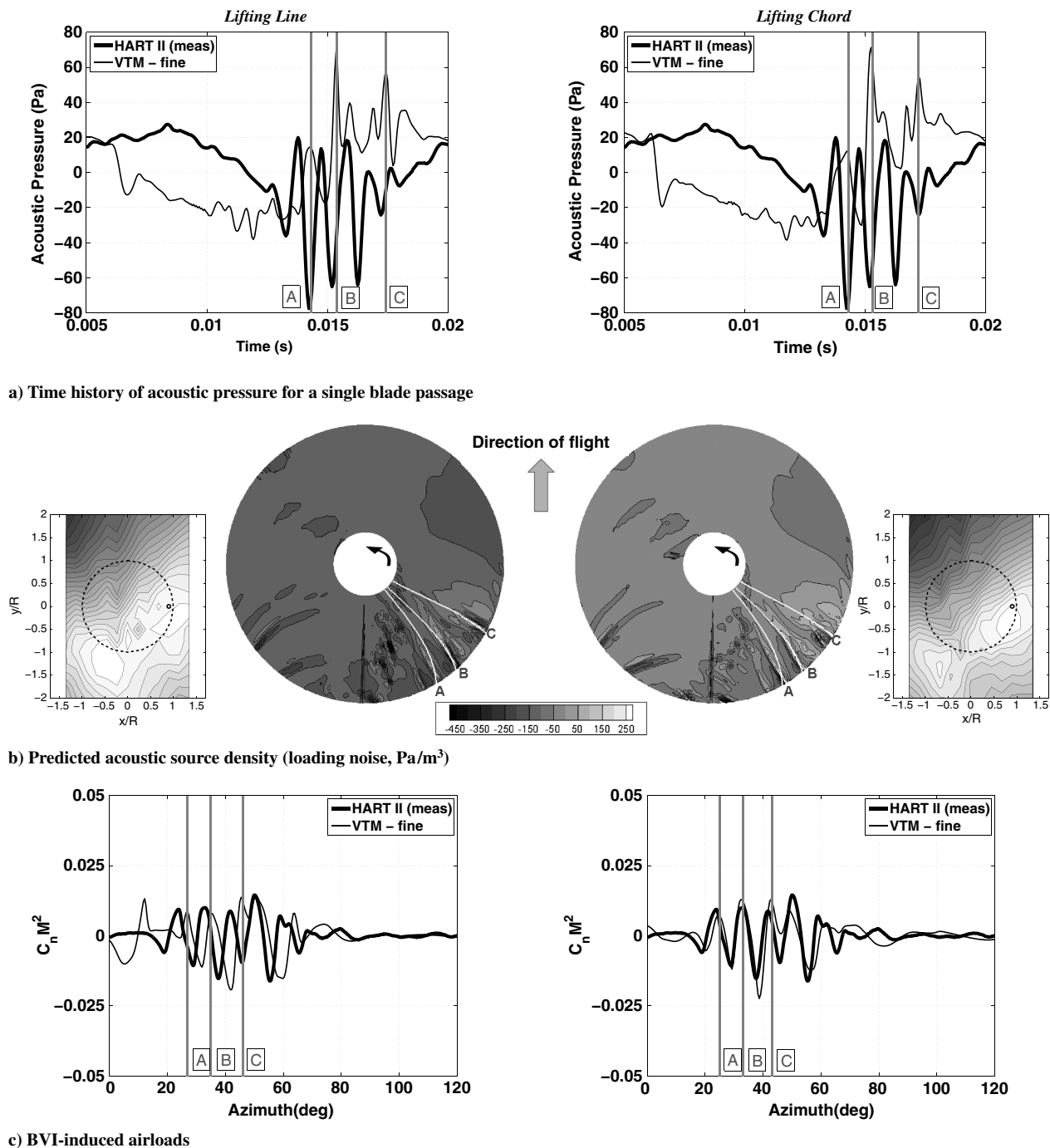
Fig. 24 Time history of acoustic pressure for one blade passage and the corresponding BVI-induced airloads and source density distribution on the rotor for an observer (marked by small circle) located at the experimentally measured SPL maximum on the advancing side of the rotor (HART II MV case). Numerical results are for the fine computational resolution.
