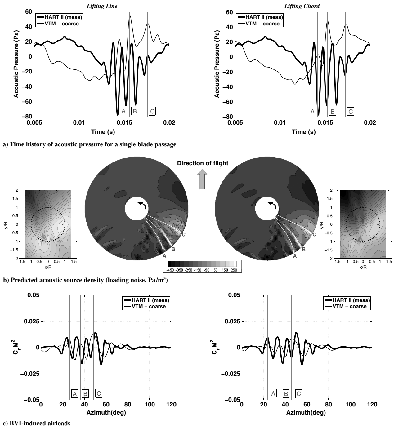
Fig. 22 Time history of acoustic pressure for one blade passage and the corresponding BVI-induced airloads and source density distribution on the rotor for an observer (marked by small circle) located at the experimentally measured SPL maximum on the advancing side of the rotor (HART II MV case). Numerical results are for the coarse computational resolution.
