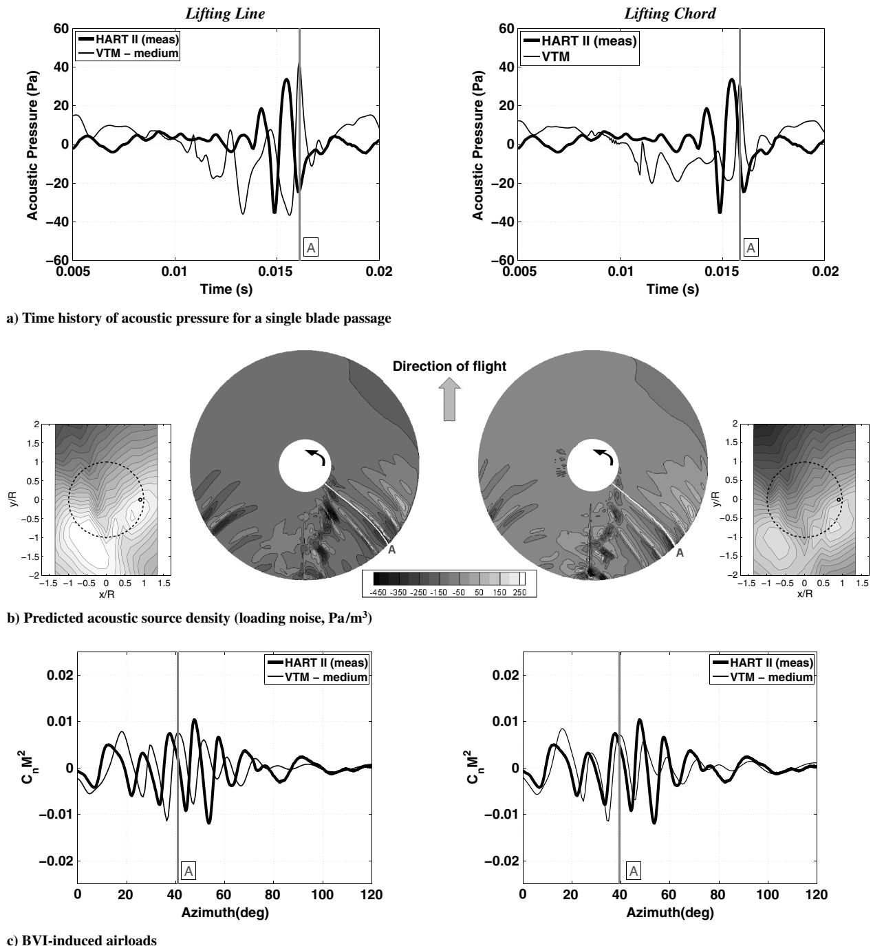
Fig. 9 Time history of acoustic pressure for one blade passage and the corresponding BVI-induced airloads and source density distribution on the rotor for an observer (marked by small circle) located at the experimentally measured SPL maximum on the advancing side of the rotor (HART II BL case). Numerical results are for the medium computational resolution.
